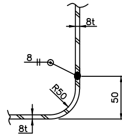
TANK STEEL WELDING DETAIL
